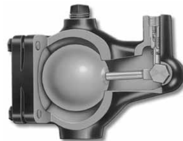
Simple Lever APCO Series #55
