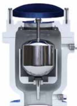
Air/Vacuum Valve Series 150
