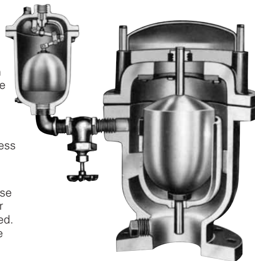
CUSTOM DUPLEX BODY COMBINATION APCO Series #1800
