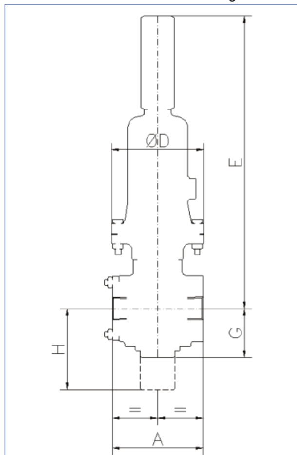
UBAN threaded valve dimensional drawing
