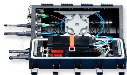
OptiSheath® Sealed Terminal, UCA Series, 6 OptiTap® Connector adapters, 6 pigtails, 2 mechanical ports, wall bracket
