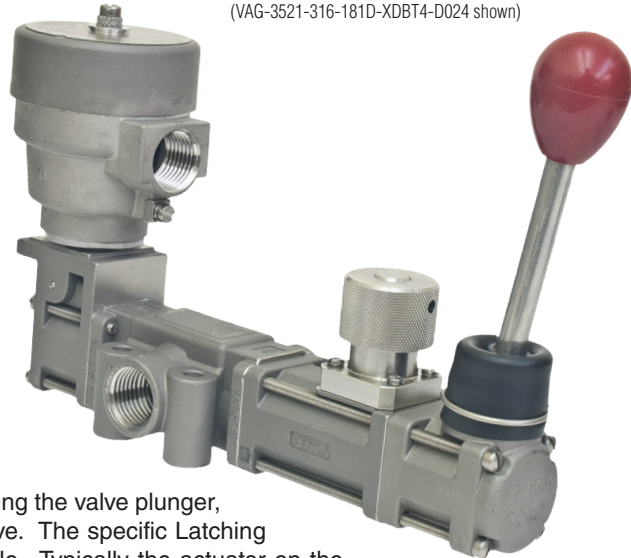
Latching/Manual Reset Three-Way Valve, Solenoid Actuated. (VAG-3521-316-181D-XDBT4-D024 shown)
