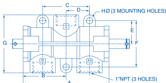
3/4" - 1" Body
