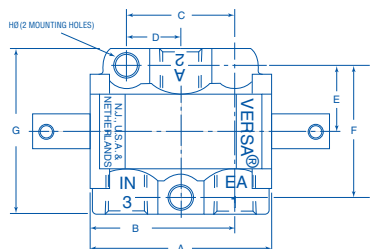
1/4" - 1/2" Body
